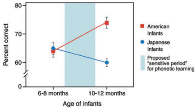
Fig. 3. Effects of age on discrimination of the American English /r-la/ phonetic contrast by American and Japanese infants at 6–8 and 10–12 months of age. Mean percent correct scores are shown with standard errors indicated (adapted from Kuhl et al., 2006).
